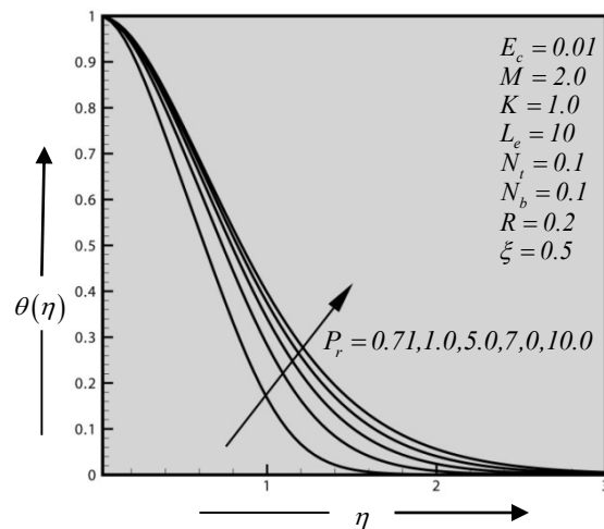
Figure 10. Temperature distribution for different values of Prandtl number ( P_r ).
