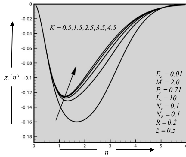
Figure 8.Secondary velocity distribution for different values of Radiation Parameter ( K ).
