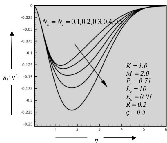
Figure 7. Secondary velocity distribution for different values of Brownian and Thermophoresis parameter ( N_b & N_t ).
