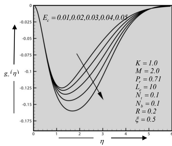
Figure 6. Secondary velocity distribution for different values of Eckert Number ( E_c ).
