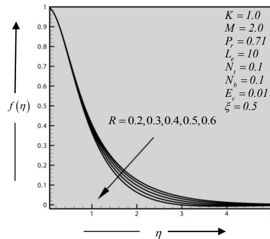
Figure 3. Primary velocity distribution for different values of Rotational parameter ( R ).
