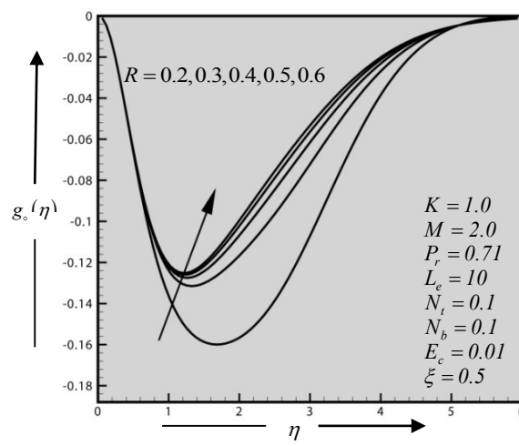
Figure 5. Secondary velocity distribution for different values of Rotational parameter ( R ).
