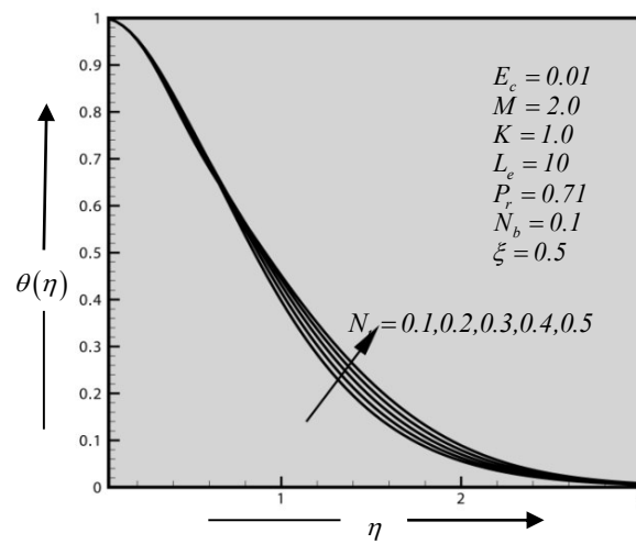
Figure 11. Temperature distribution for different values of Thermophoresis parameter ( N_t ).
