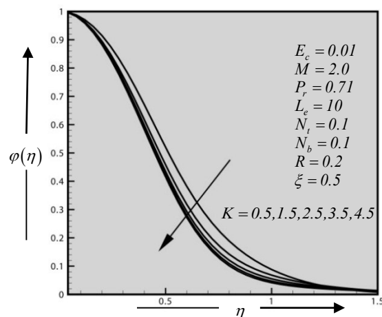
Figure 12. Concentration distribution for different values of Radiation Parameter ( K ).
