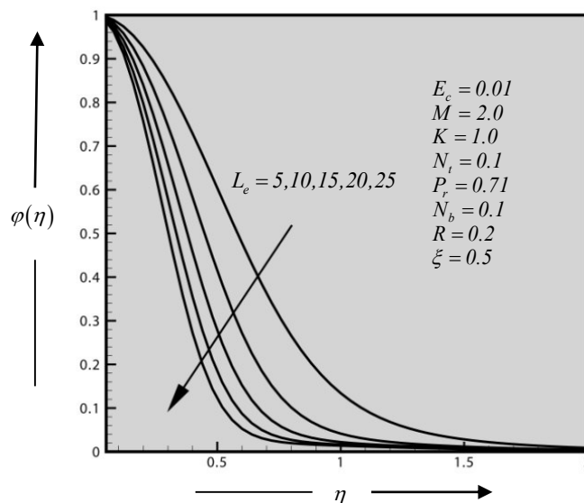
Figure 14. Concentration distribution for different values of Lewis number ( L_e ).
