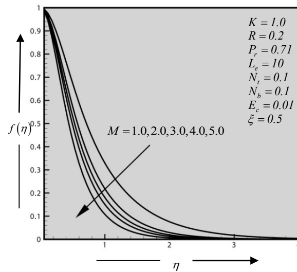
Figure 2. Primary velocity distribution for different values of Magnetic parameter ( M ).
