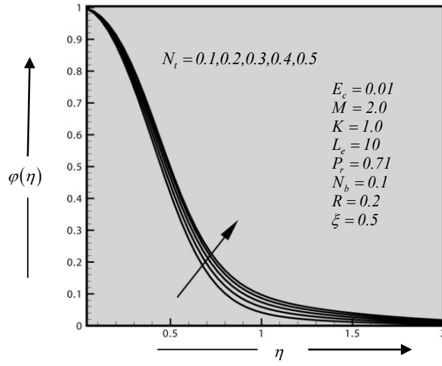
Figure 13. Concentration distribution for different values of Thermophoresis parameter ( N_t )
