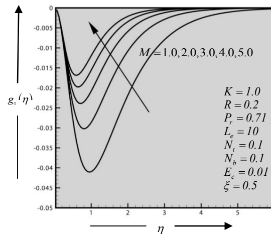
Figure 4. Secondary velocity distribution for different values of Magnetic parameter ( M ).
